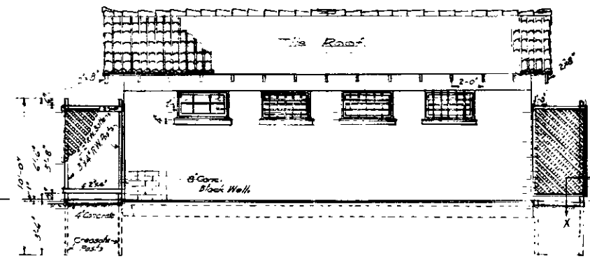
SIDE ELEVATION Scale 1/2" = 1'
