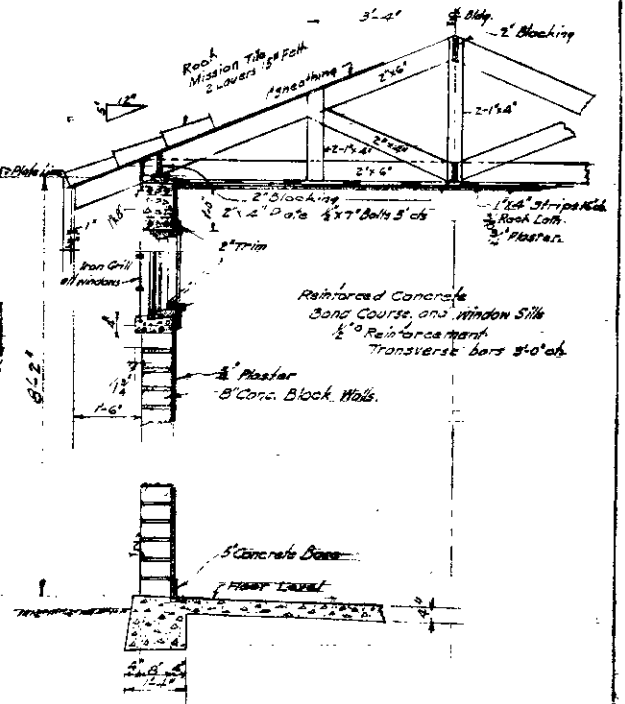
PART SECTION Scale 1/2" = 1'
