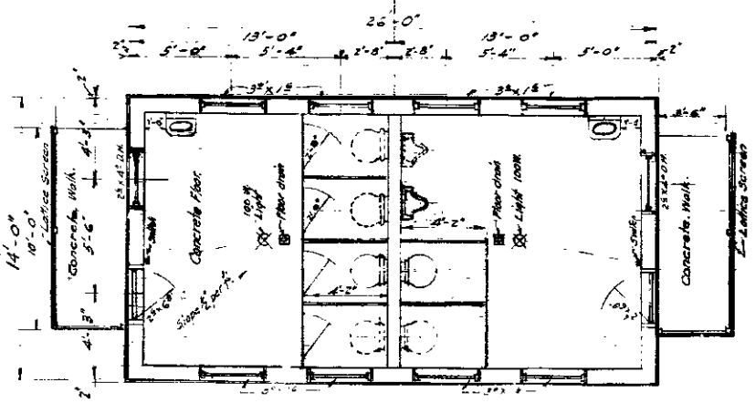
PLAN Scale 1/2" = 1'
